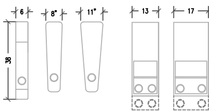
STRAIGHT & WEDGE ARMS
