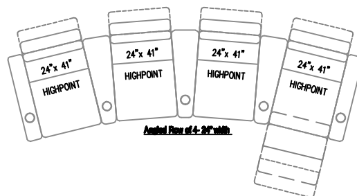
TOP VIEW OF HIGHPOINT CONSOLE
